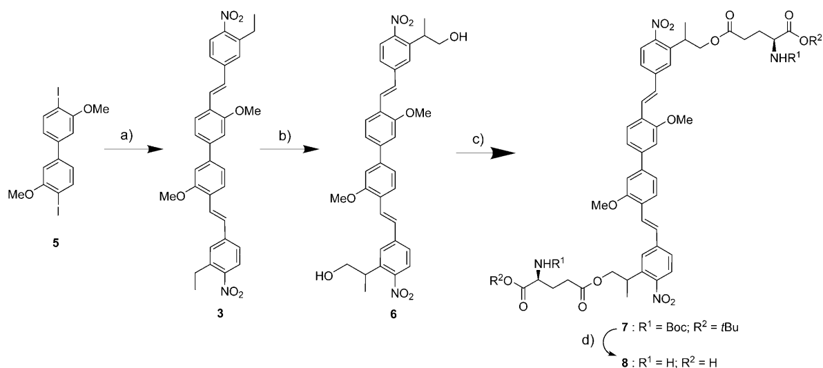
Scheme 1. Synthesis of caged glutamate 8 (BNSMB-Glu). a) Xylenes, Pd(OAc) 2 , Et 3 N, tri- o -tolylphosphine, 3-ethyl-4-nitrostyrene; 5 days, 140 °C, 68 %; b) t BuOK/ t BuOH, paraformaldehyde, dimethylsulfoxide (DMSO), 80 °C, 3 h; c) Boc-L-Glu-O- t Bu (boc = tert -butoxycarbonyl), 4-dimethylaminopyridine (DMAP), dicyclohexylcarbodiimide (DCC), CH 2 Cl 2 , room temperature, 2 h; d) 20 % trifluoroacetic acid (TFA), CH 2 Cl 2 , room temperature, 6 h.
