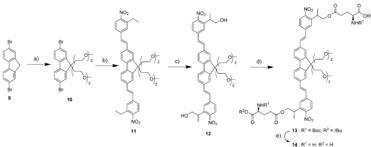
Scheme 2. Synthesis of caged glutamate 14 (BNSF-Glu). a) NaH, N,N -dimethylformamide, 1-bromo-2-(2-methoxyethoxy)ethane; b) xylenes, Pd(OAc) 2 , Et 3 N, tri- o -tolylphosphine, 3-ethyl-4-nitrostyrene, 5 days, 140 °C, 68 %; c) t BuOK/ t BuOH, paraformaldehyde, DMSO, 80 °C 3 h, 20 %; d) Boc-L-Glu-O- t Bu, DMAP, DCC, CH 2 Cl 2 , room temperature, 2 h; e) 20 % TFA, CH 2 Cl 2 , room temperature, 6 h.
